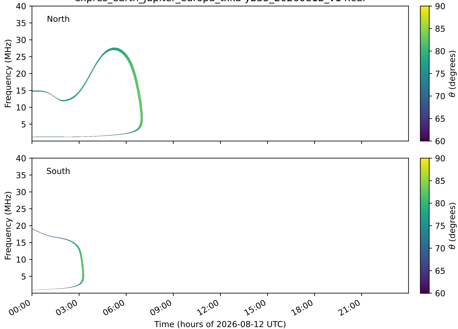
expres_earth_jupiter_europa_txka-y235_20260812_v14.cdf
