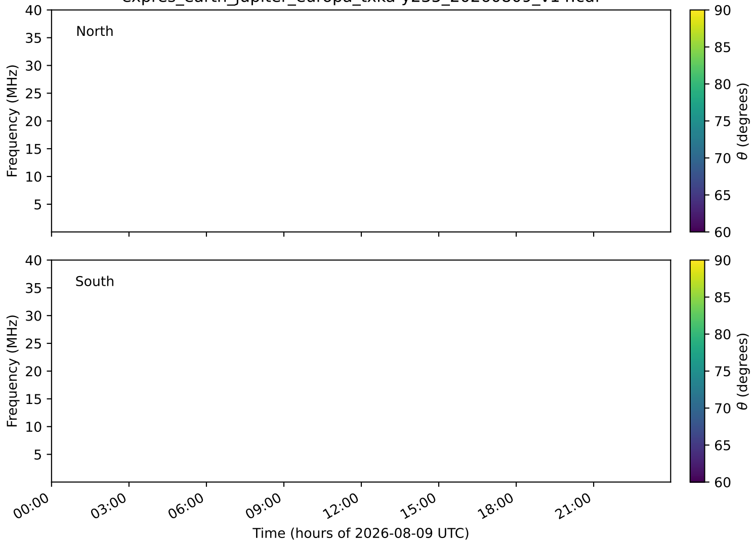
expres_earth_jupiter_europa_txka-y235_20260809_v14.cdf
