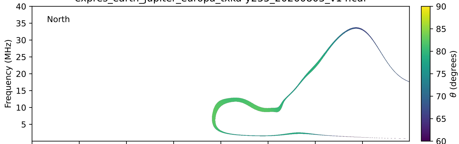
expres_earth_jupiter_europa_txka-y235_20260803_v14.cdf
