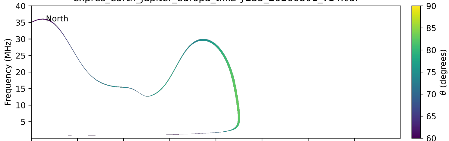
expres_earth_jupiter_europa_txka-y235_20260801_v14.cdf
