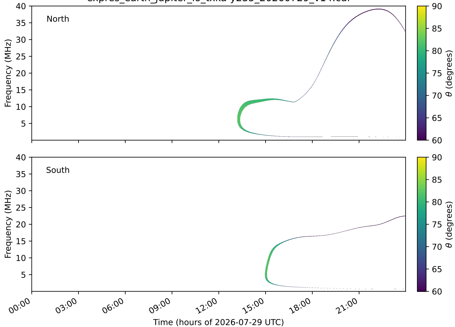
expres_earth_jupiter_io_txka-y235_20260729_v14.cdf
