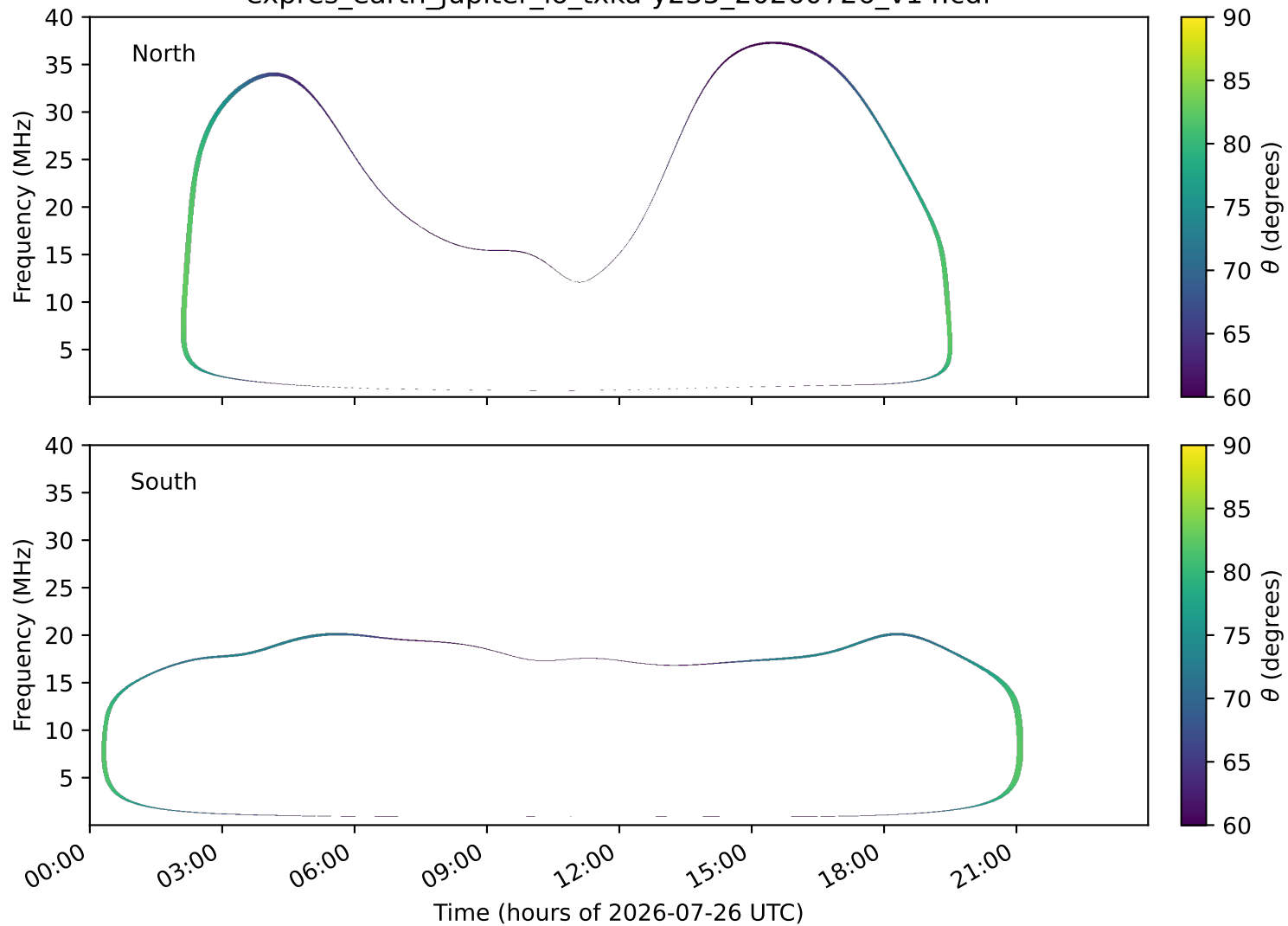
expres_earth_jupiter_io_txka-y235_20260726_v14.cdf
