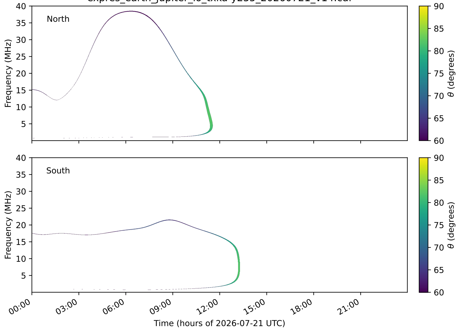
expres_earth_jupiter_io_txka-y235_20260721_v14.cdf
