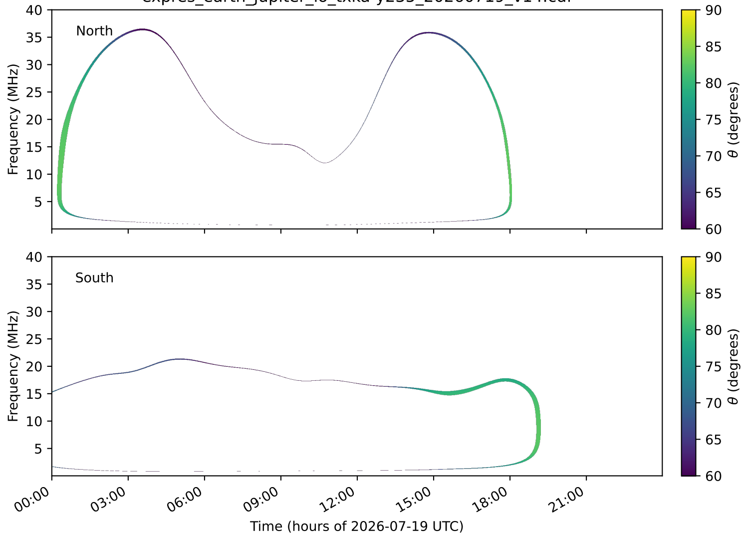
expres_earth_jupiter_io_txka-y235_20260719_v14.cdf
