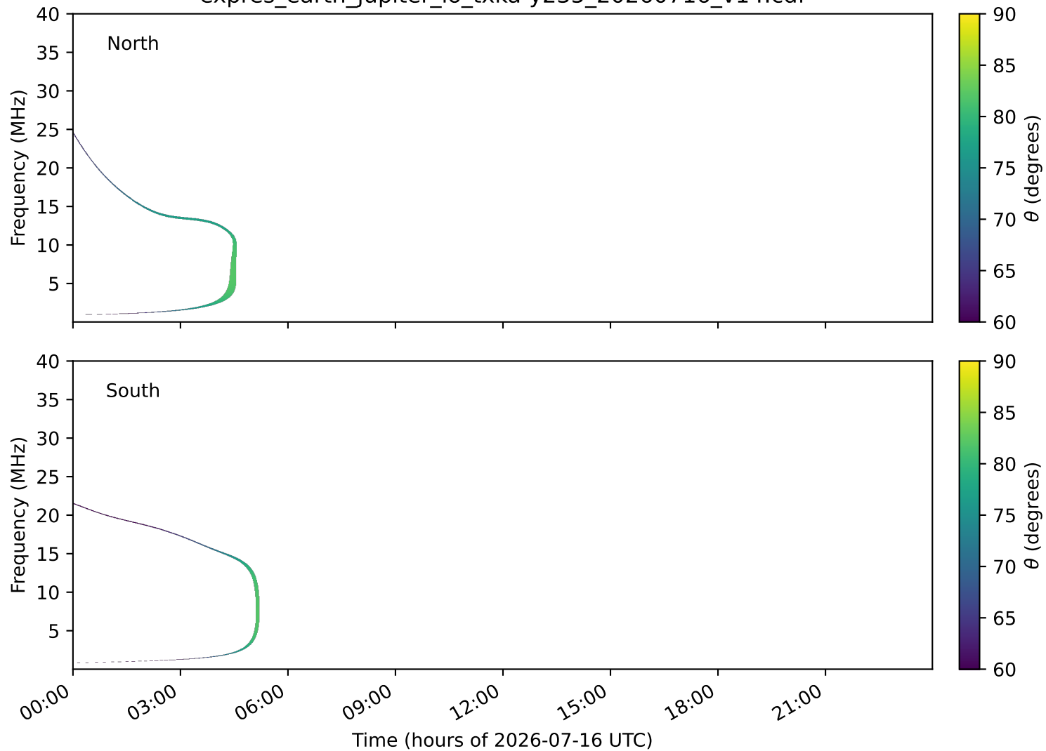
expres_earth_jupiter_io_txka-y235_20260716_v14.cdf
