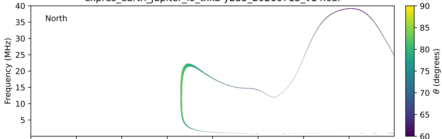
expres_earth_jupiter_io_txka-y235_20260715_v14.cdf
