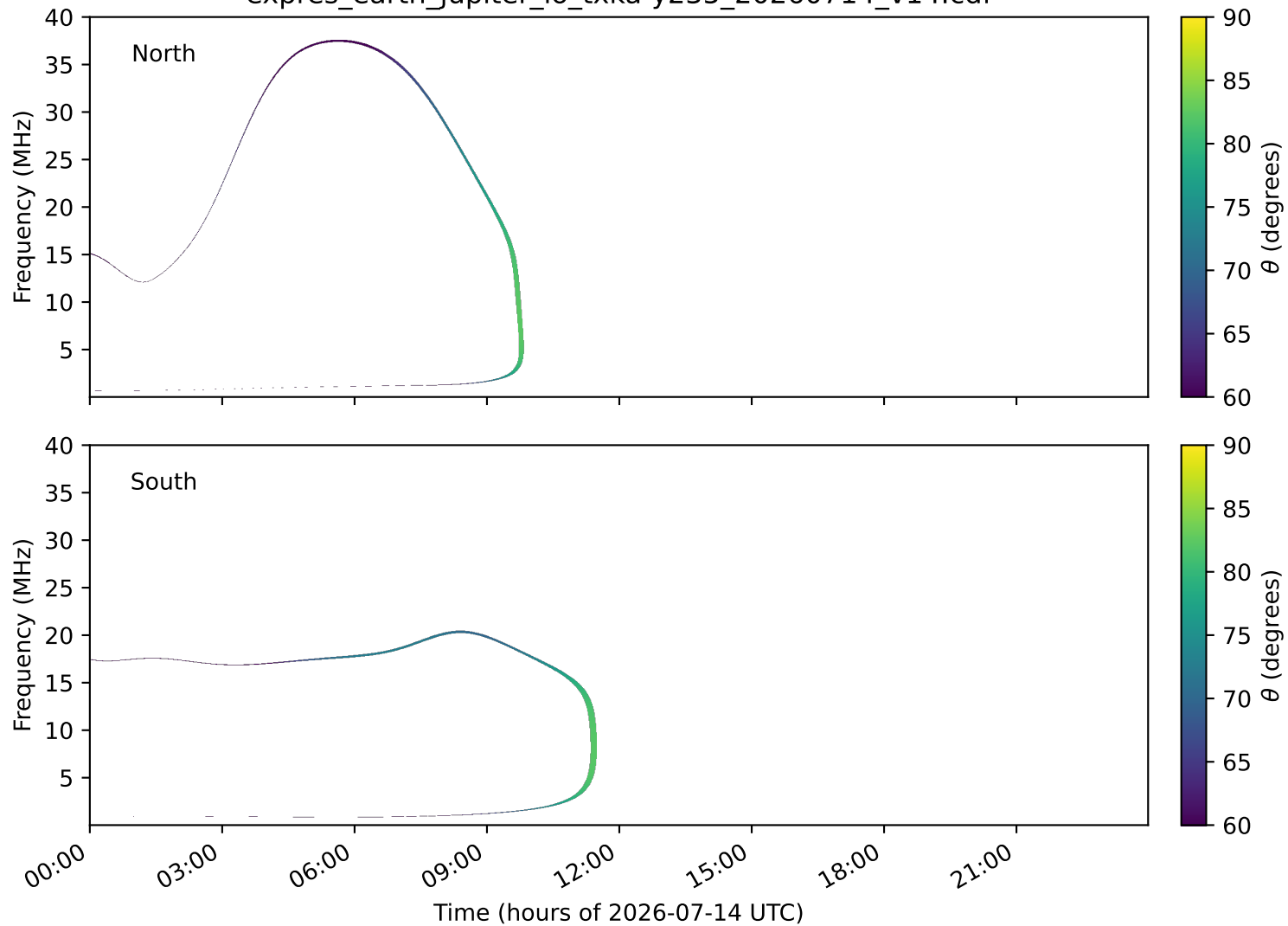
expres_earth_jupiter_io_txka-y235_20260714_v14.cdf
