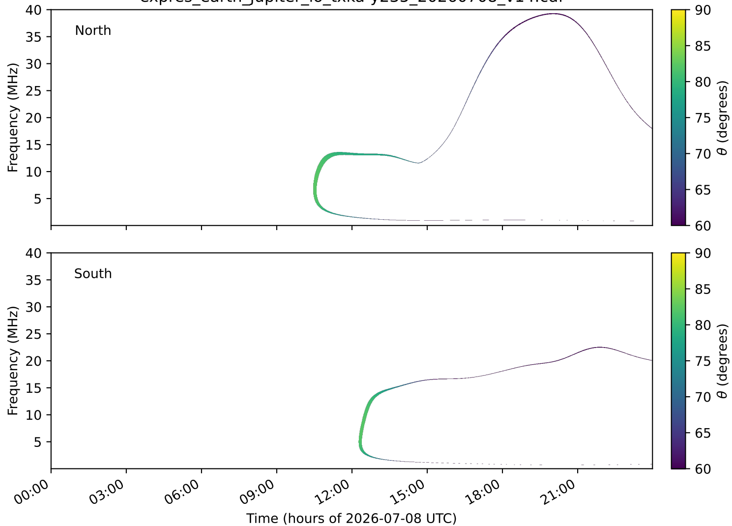
expres_earth_jupiter_io_txka-y235_20260708_v14.cdf
