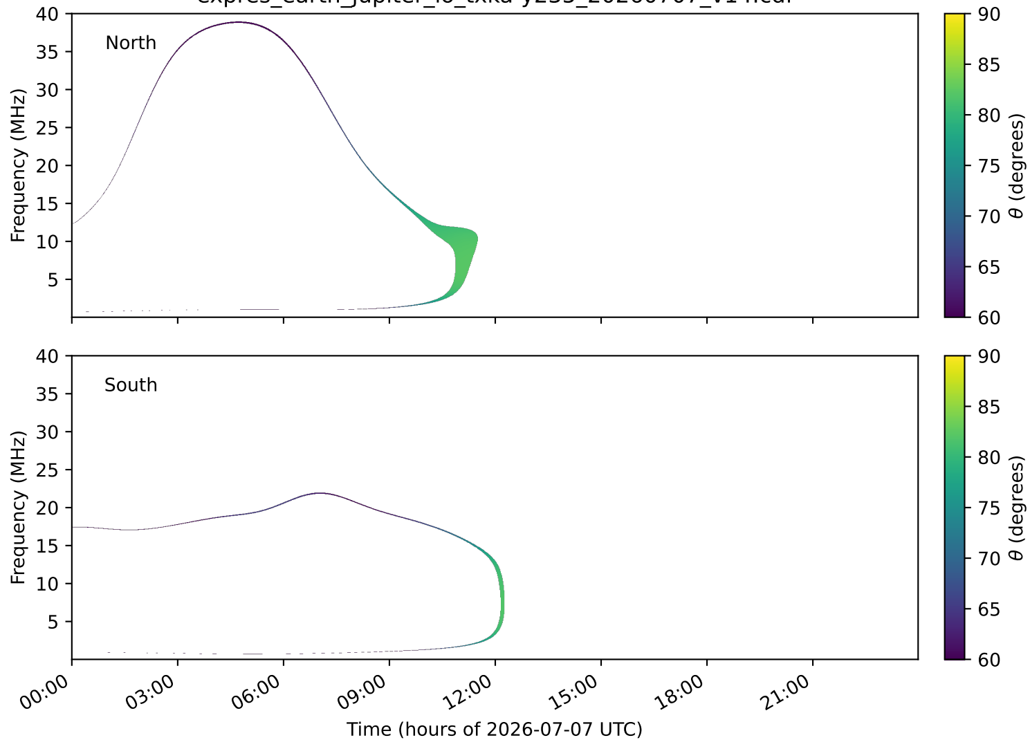
expres_earth_jupiter_io_txka-y235_20260707_v14.cdf
