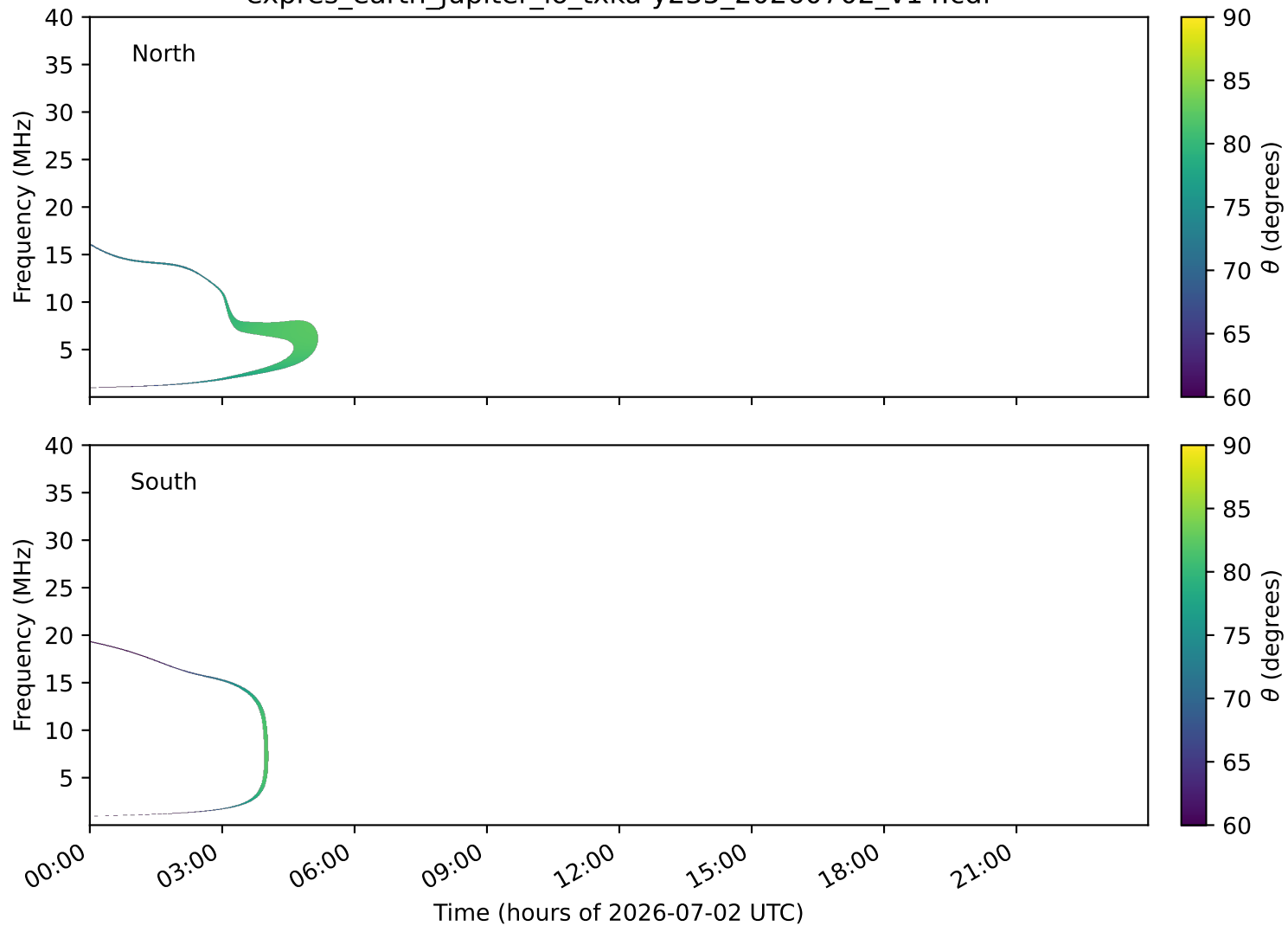
expres_earth_jupiter_io_txka-y235_20260702_v14.cdf
