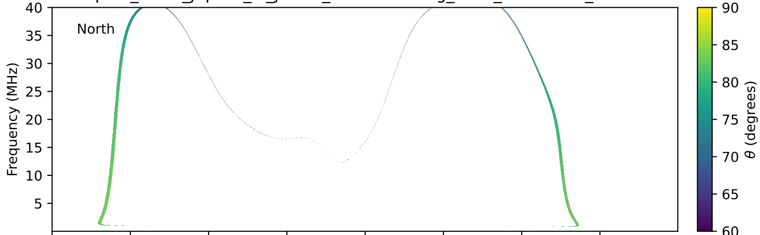
expres_earth_jupiter_io_jrm33_lossc-wid1deg_3kev_20260726_v11.cdf
