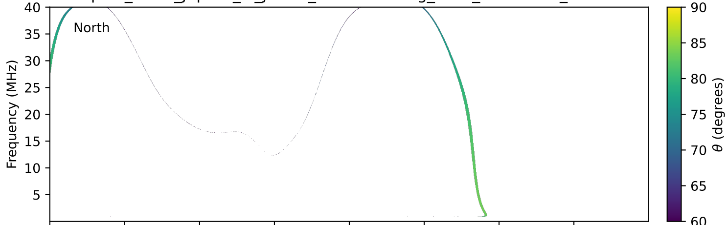
expres_earth_jupiter_io_jrm33_lossc-wid1deg_3kev_20260705_v11.cdf
