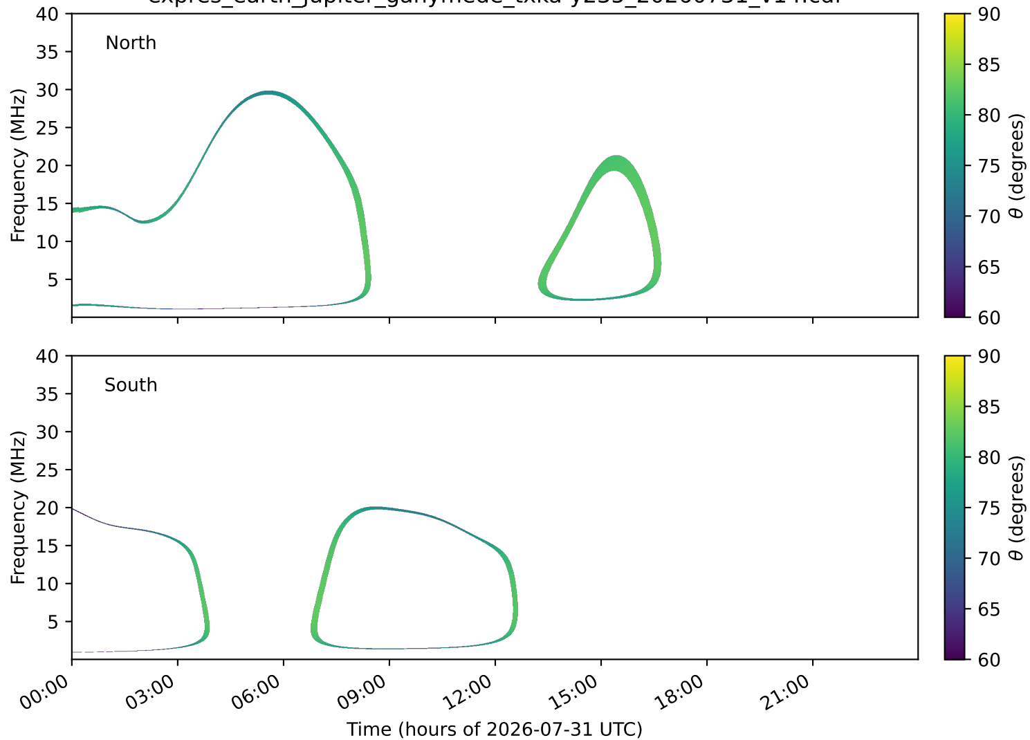
expres_earth_jupiter_ganymede_txka-y235_20260731_v14.cdf
