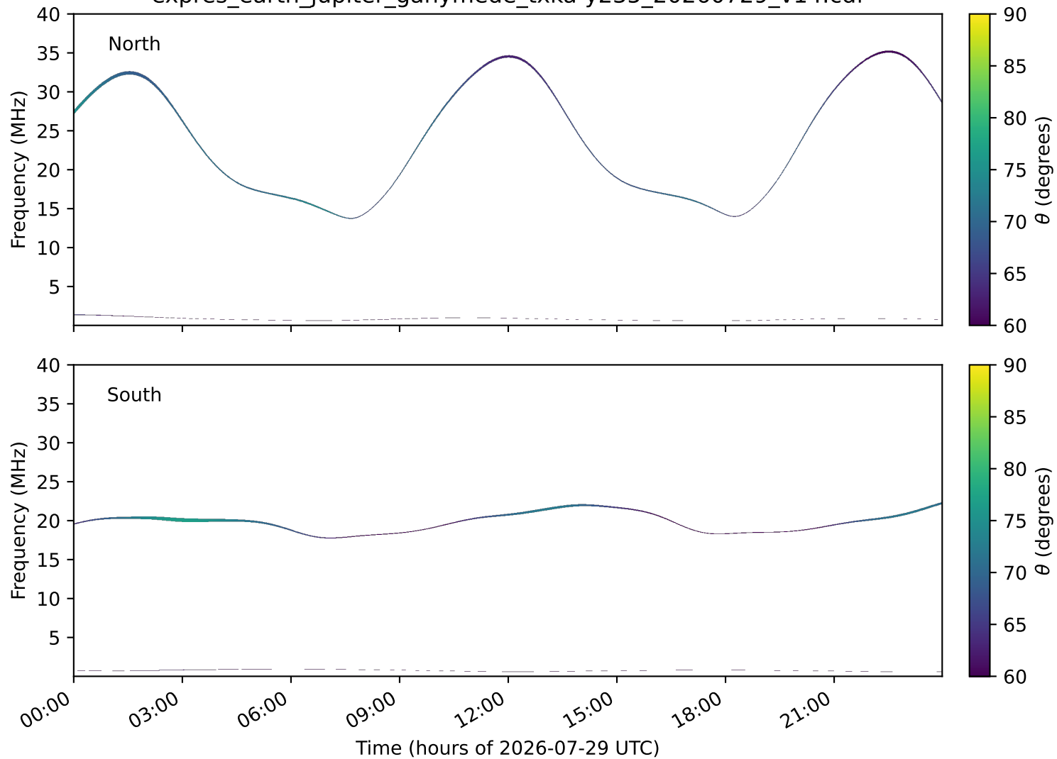
expres_earth_jupiter_ganymede_txka-y235_20260729_v14.cdf
