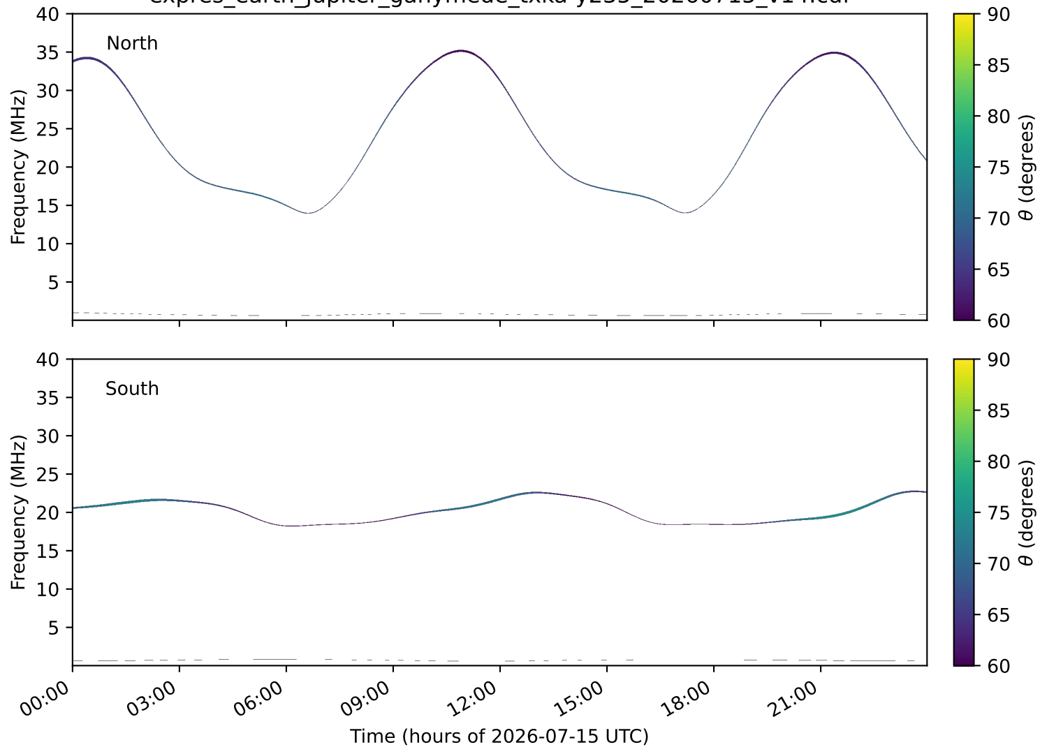
expres_earth_jupiter_ganymede_txka-y235_20260715_v14.cdf
