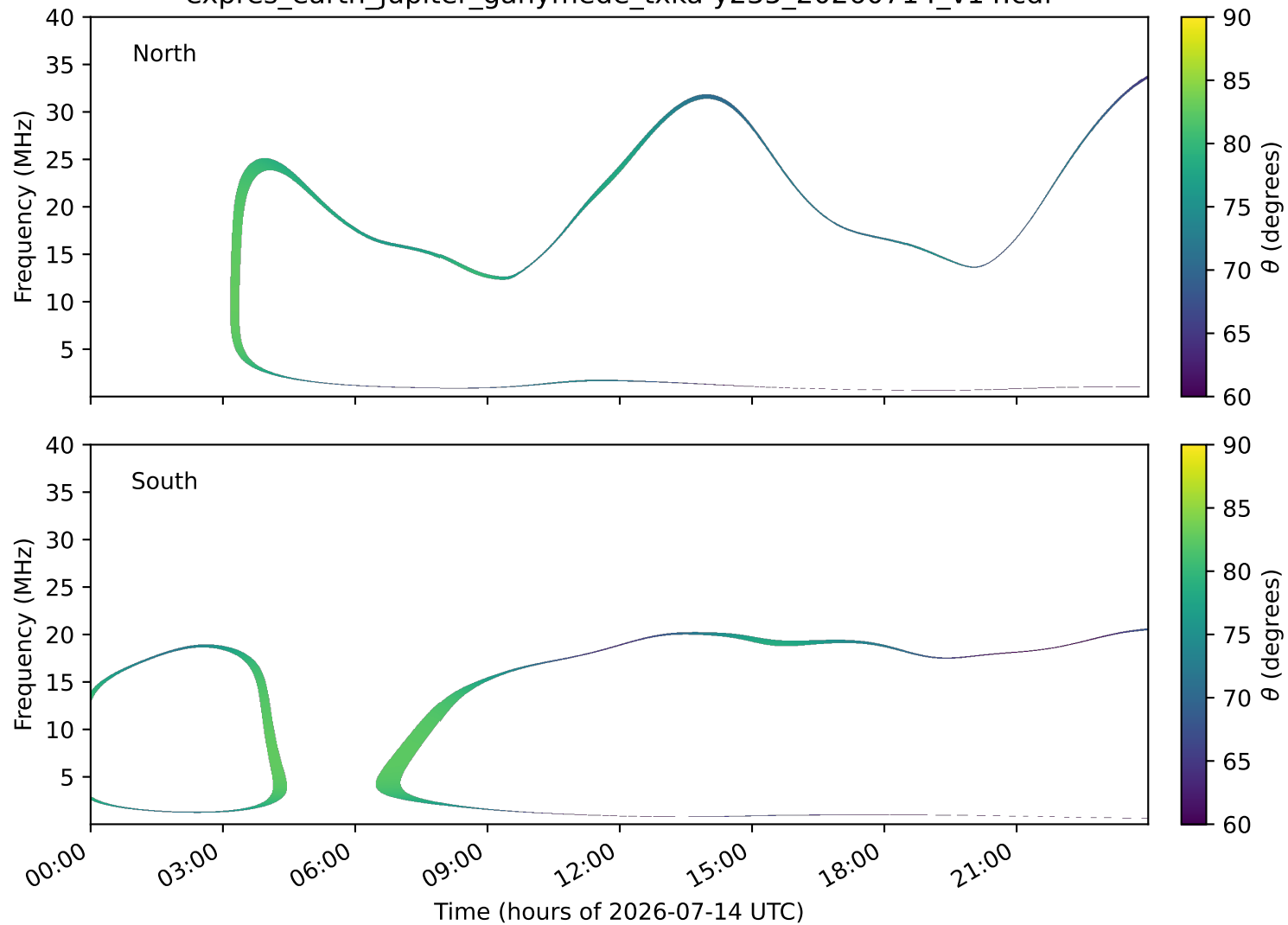
expres_earth_jupiter_ganymede_txka-y235_20260714_v14.cdf
