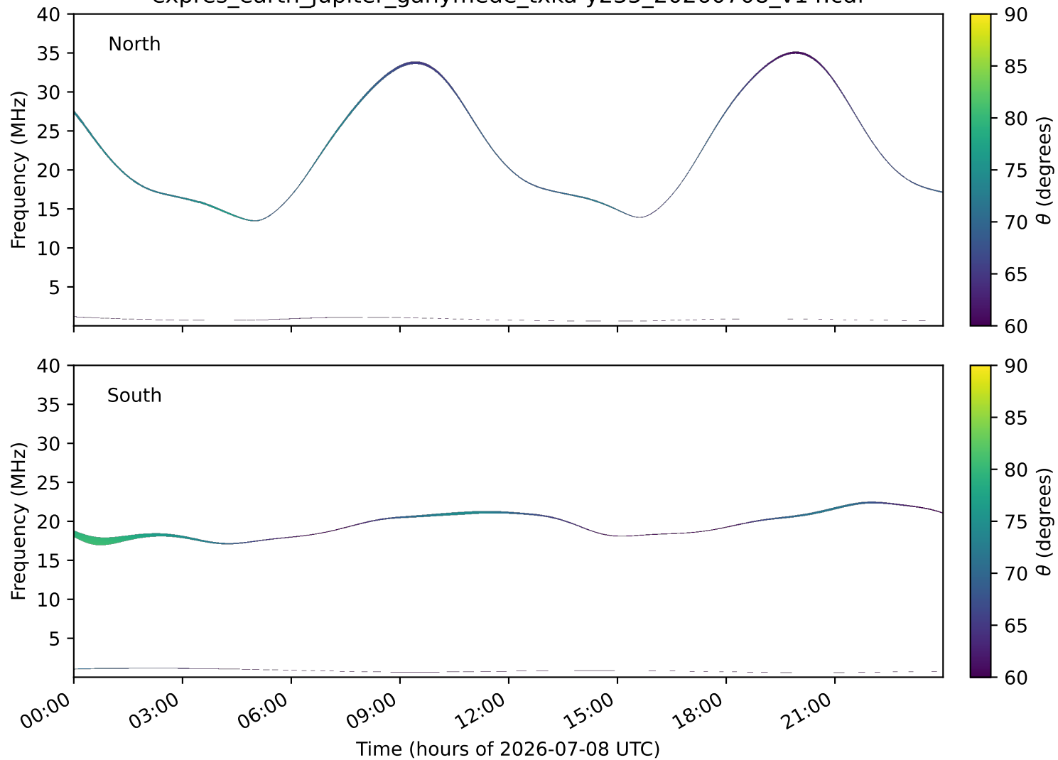
expres_earth_jupiter_ganymede_txka-y235_20260708_v14.cdf
