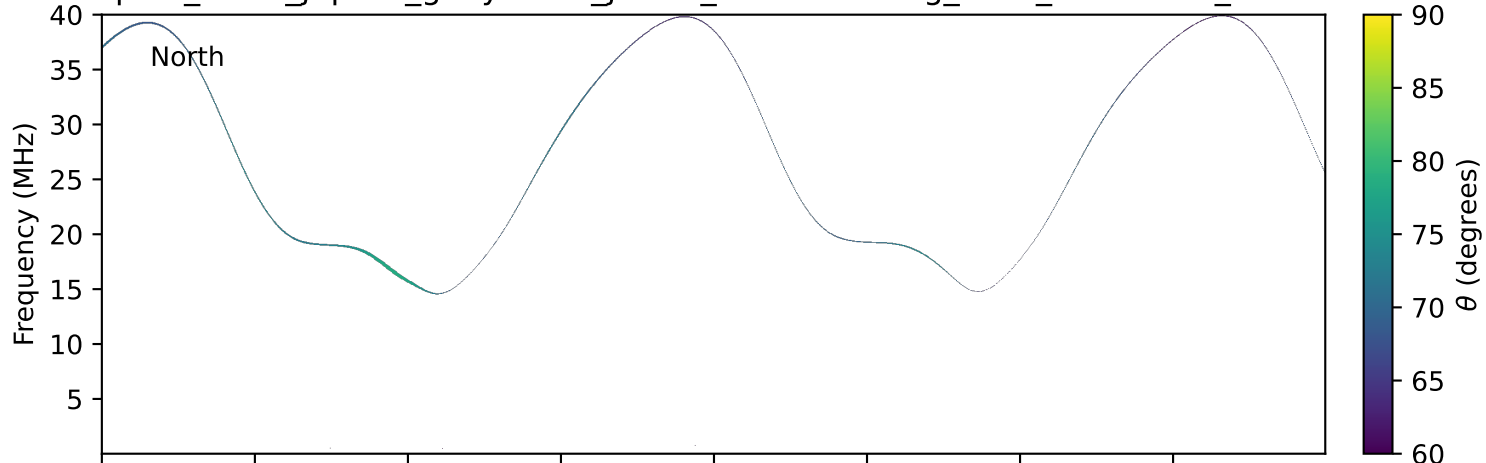
expres_earth_jupiter_ganymede_jrm33_lossc-wid1deg_3kev_20260722_v11.cdf
