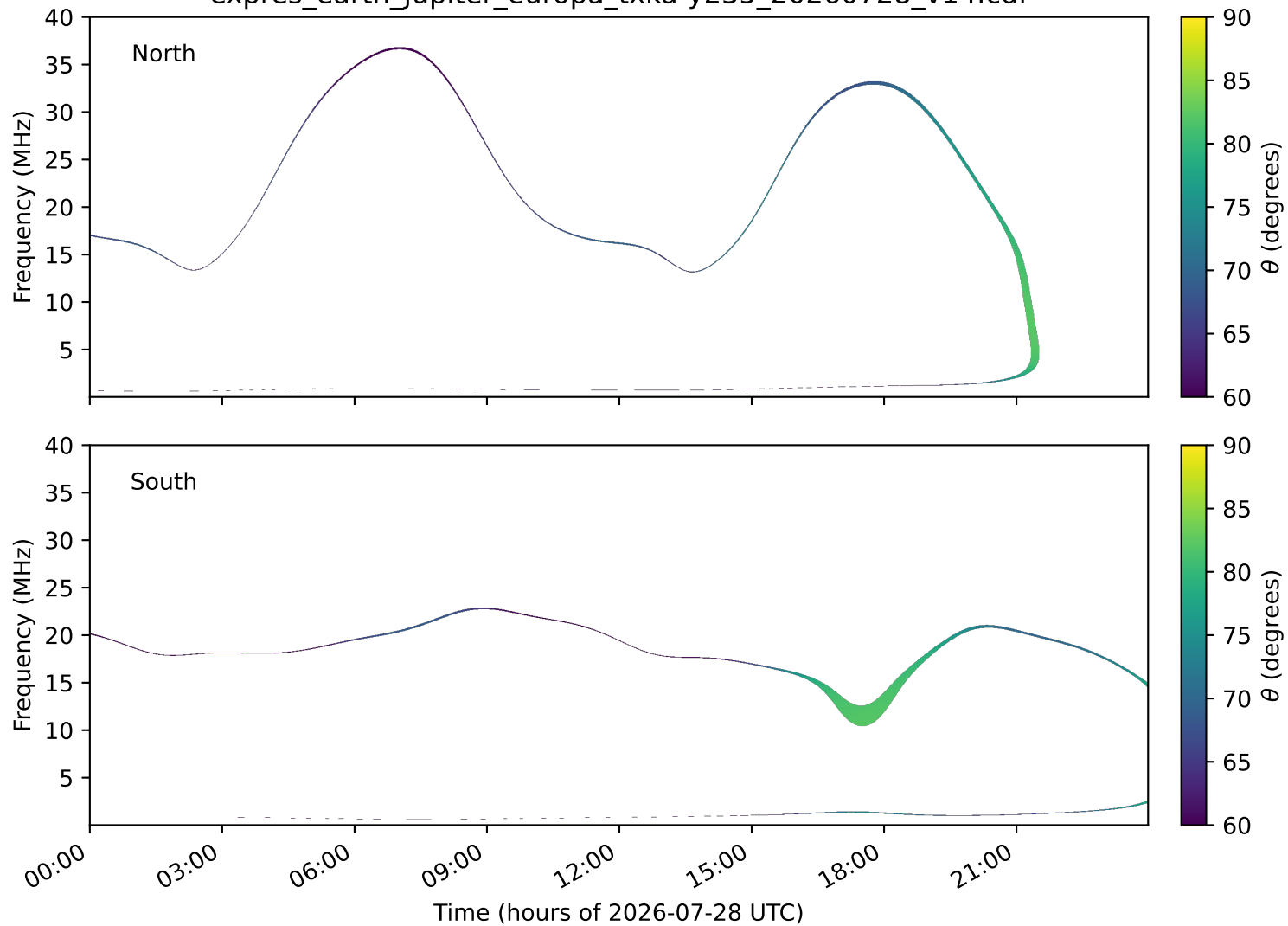
expres_earth_jupiter_europa_txka-y235_20260728_v14.cdf
