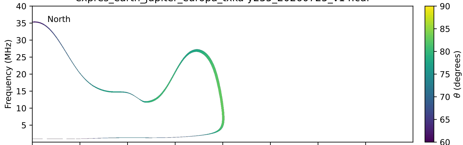
expres_earth_jupiter_europa_txka-y235_20260725_v14.cdf
