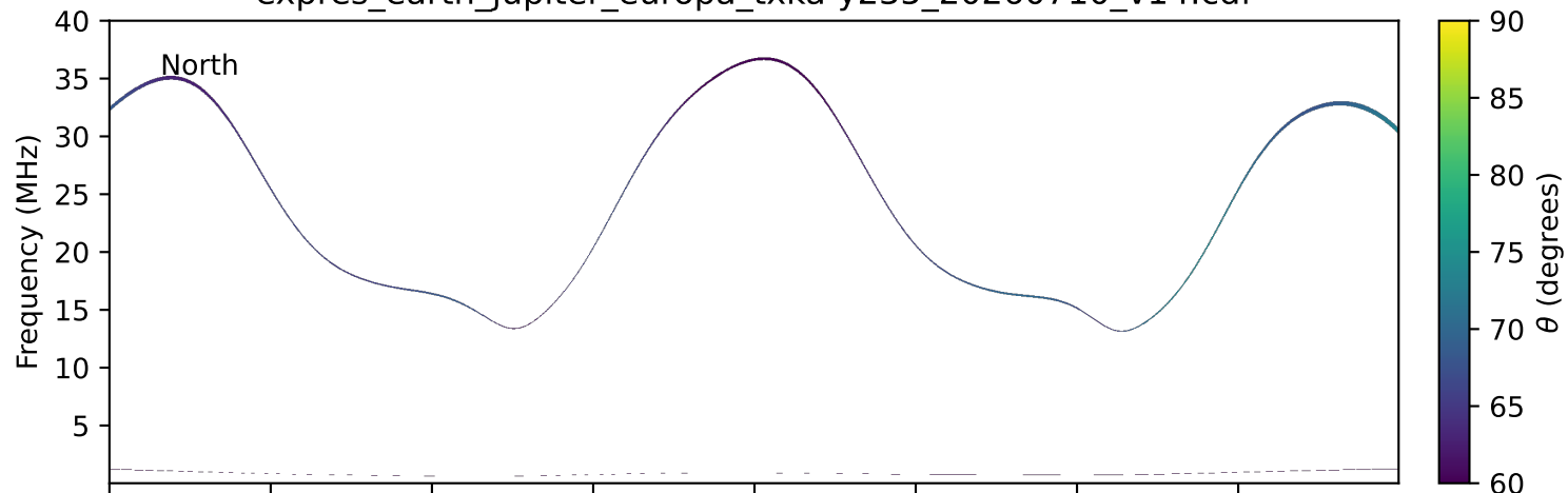
expres_earth_jupiter_europa_txka-y235_20260710_v14.cdf
