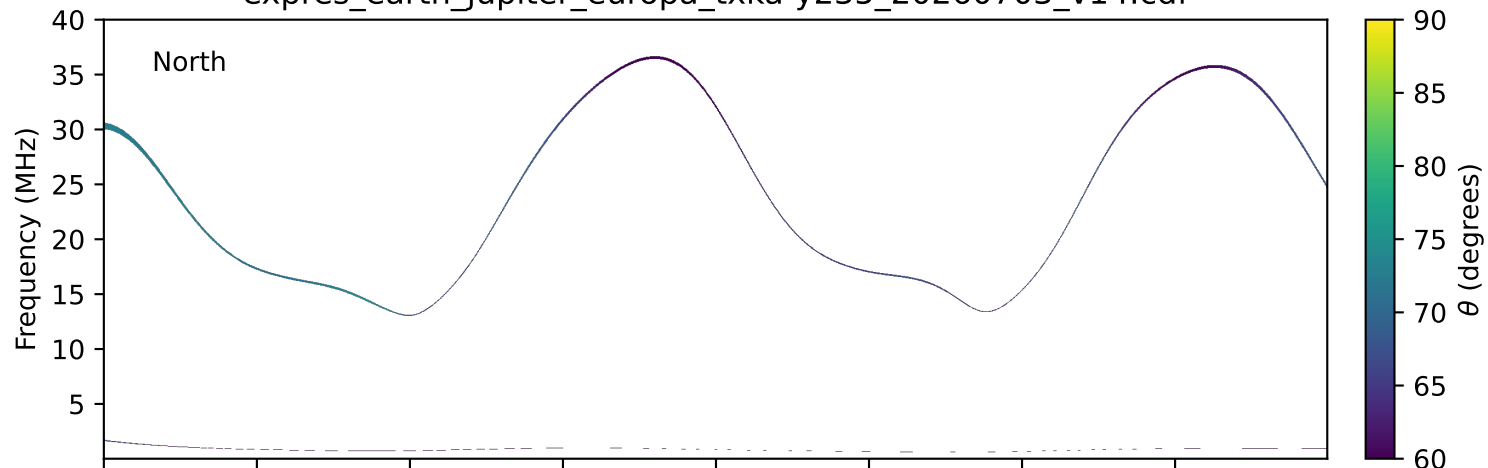
expres_earth_jupiter_europa_txka-y235_20260703_v14.cdf
