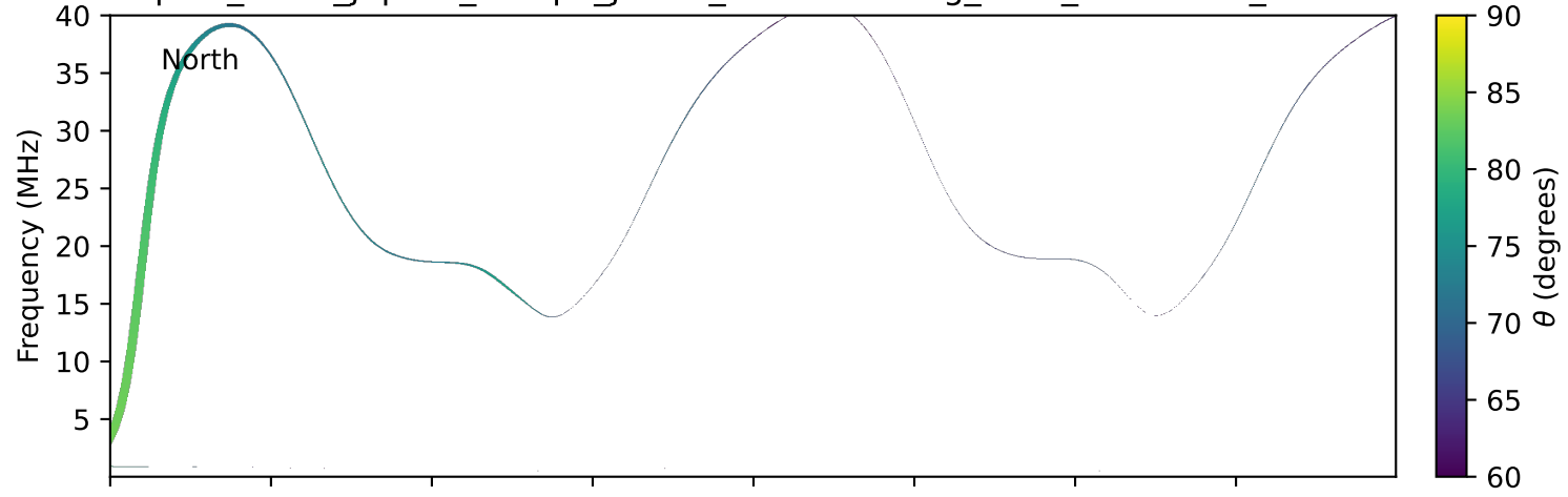
expres_earth_jupiter_europa_jrm33_lossc-wid1deg_3kev_20260724_v11.cdf
