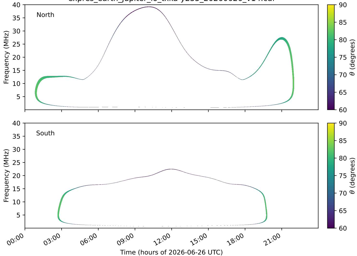
expres_earth_jupiter_io_txka-y235_20260626_v14.cdf
