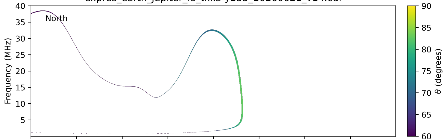
expres_earth_jupiter_io_txka-y235_20260621_v14.cdf
