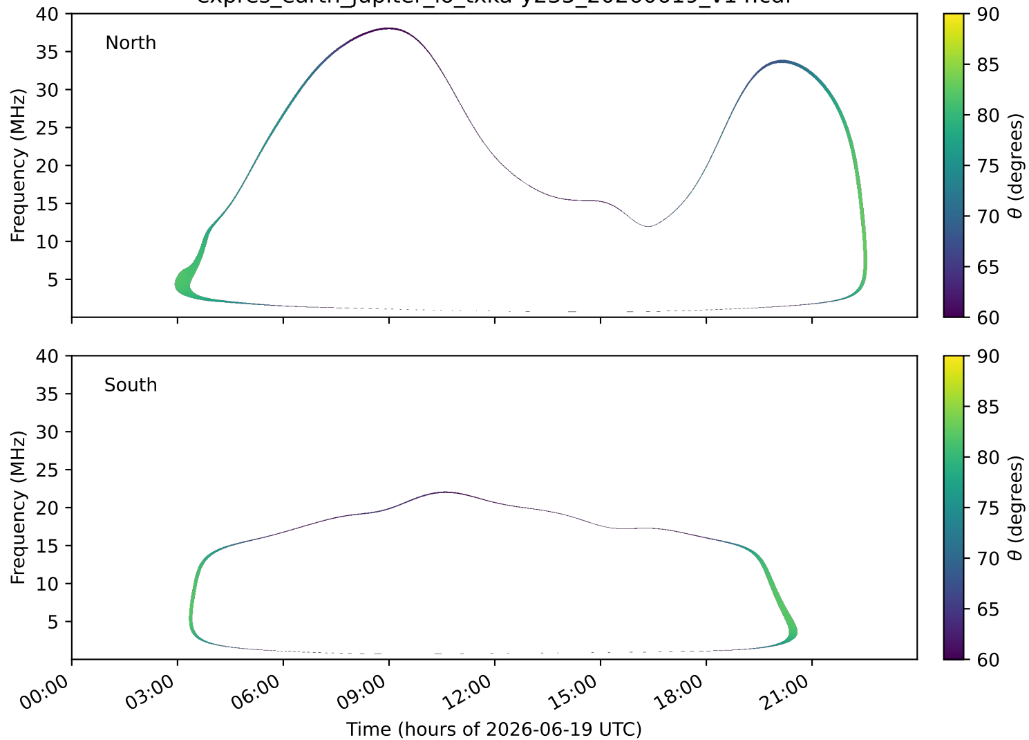
expres_earth_jupiter_io_txka-y235_20260619_v14.cdf
