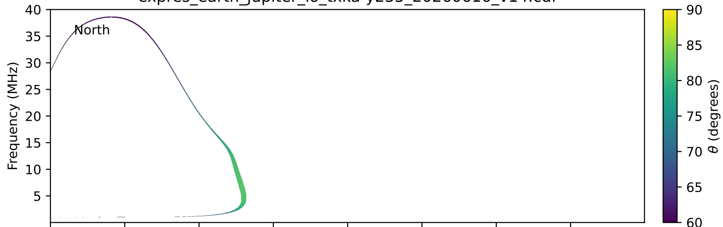
expres_earth_jupiter_io_txka-y235_20260616_v14.cdf
