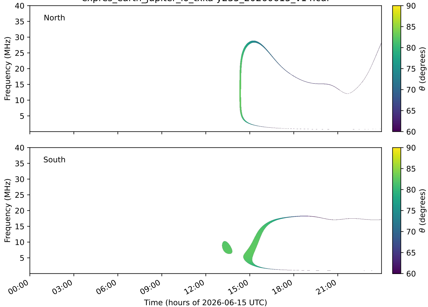
expres_earth_jupiter_io_txka-y235_20260615_v14.cdf
