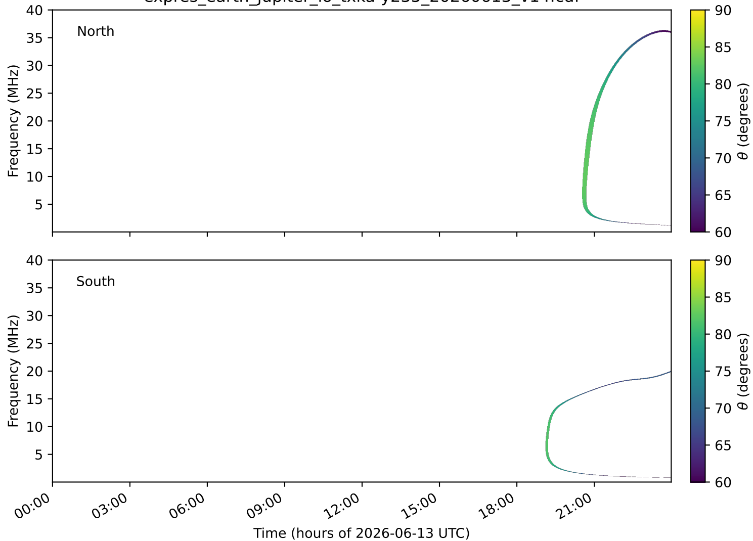
expres_earth_jupiter_io_txka-y235_20260613_v14.cdf
