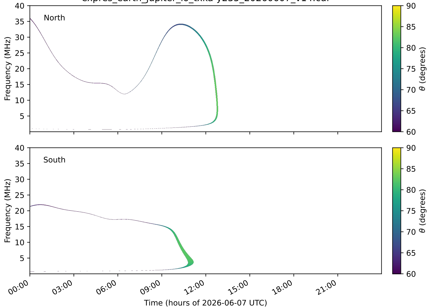
expres_earth_jupiter_io_txka-y235_20260607_v14.cdf
