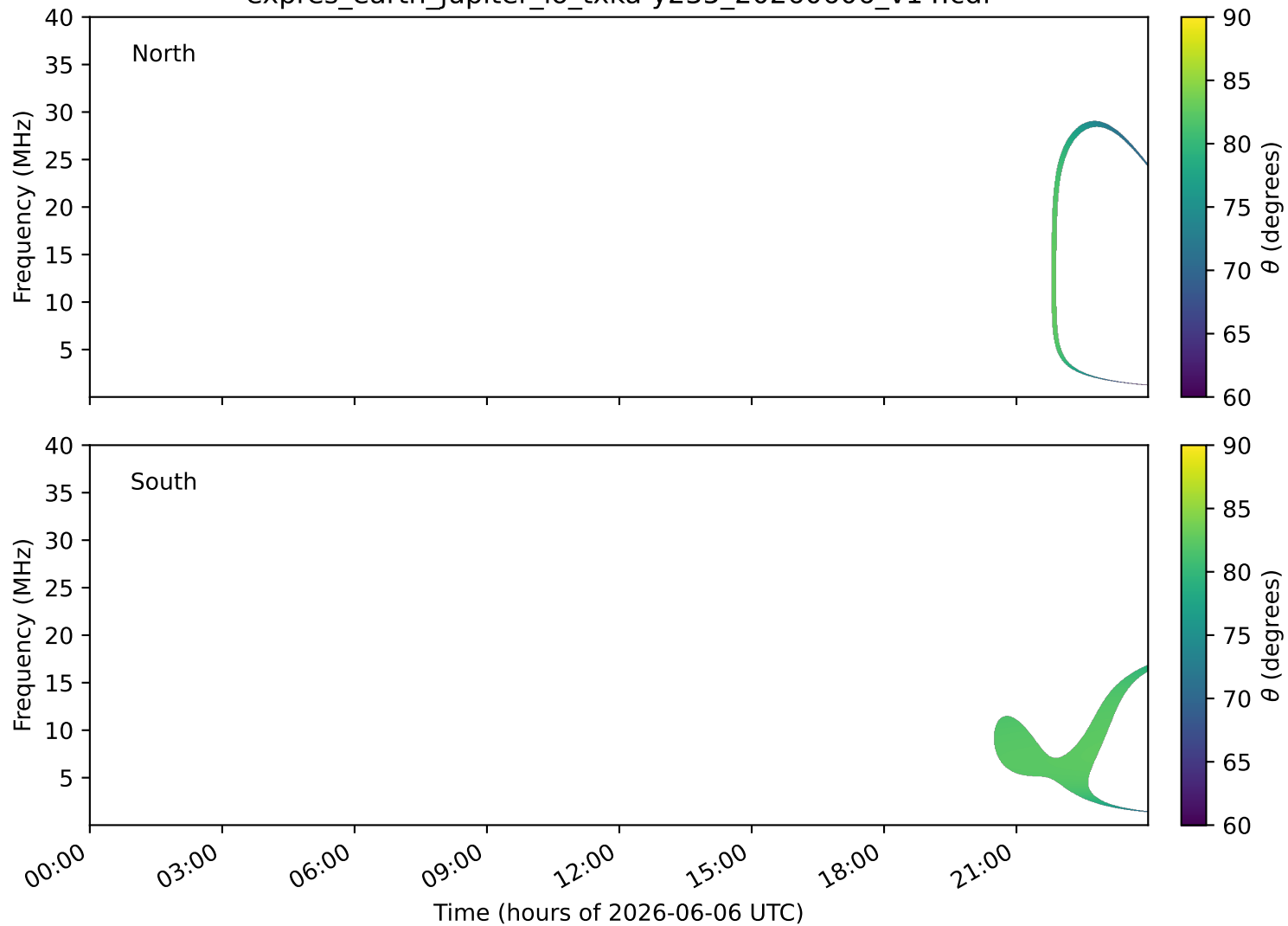
expres_earth_jupiter_io_txka-y235_20260606_v14.cdf
