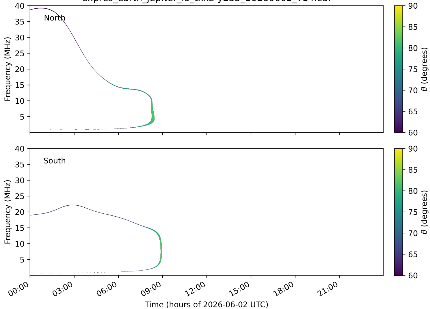
expres_earth_jupiter_io_txka-y235_20260602_v14.cdf
