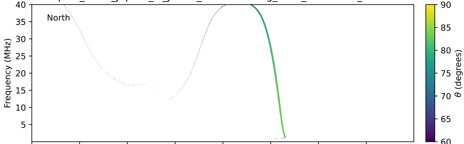
expres_earth_jupiter_io_jrm33_lossc-wid1deg_3kev_20260628_v11.cdf
