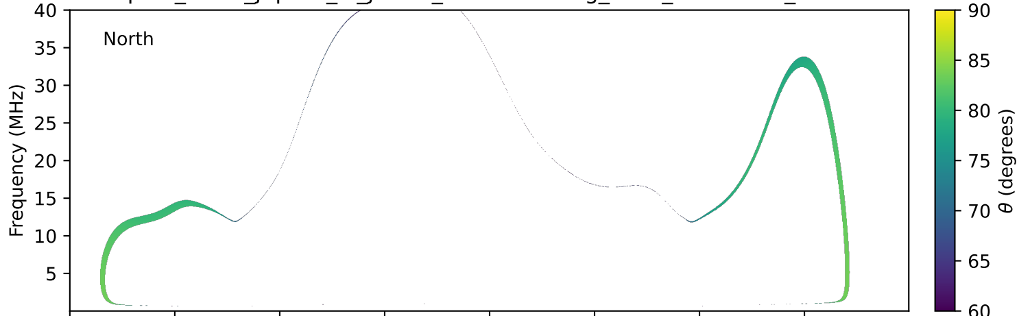
expres_earth_jupiter_io_jrm33_lossc-wid1deg_3kev_20260626_v11.cdf
