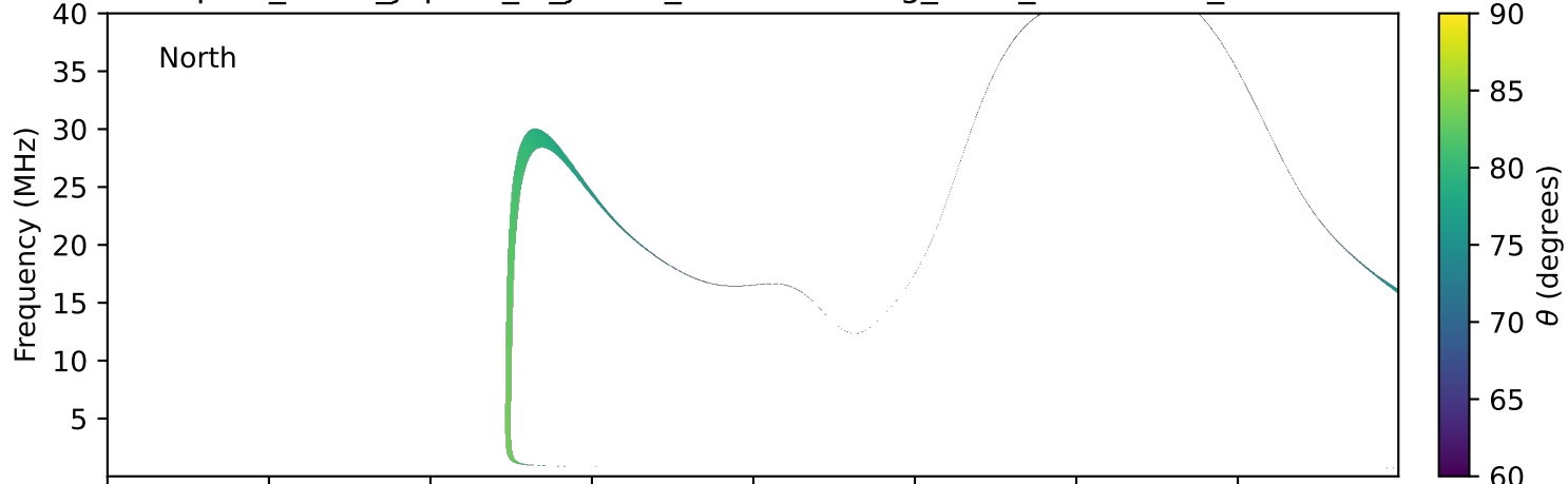
expres_earth_jupiter_io_jrm33_lossc-wid1deg_3kev_20260624_v11.cdf
