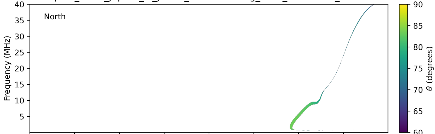
expres_earth_jupiter_io_jrm33_lossc-wid1deg_3kev_20260620_v11.cdf
