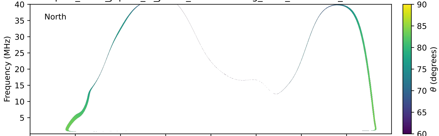
expres_earth_jupiter_io_jrm33_lossc-wid1deg_3kev_20260619_v11.cdf
