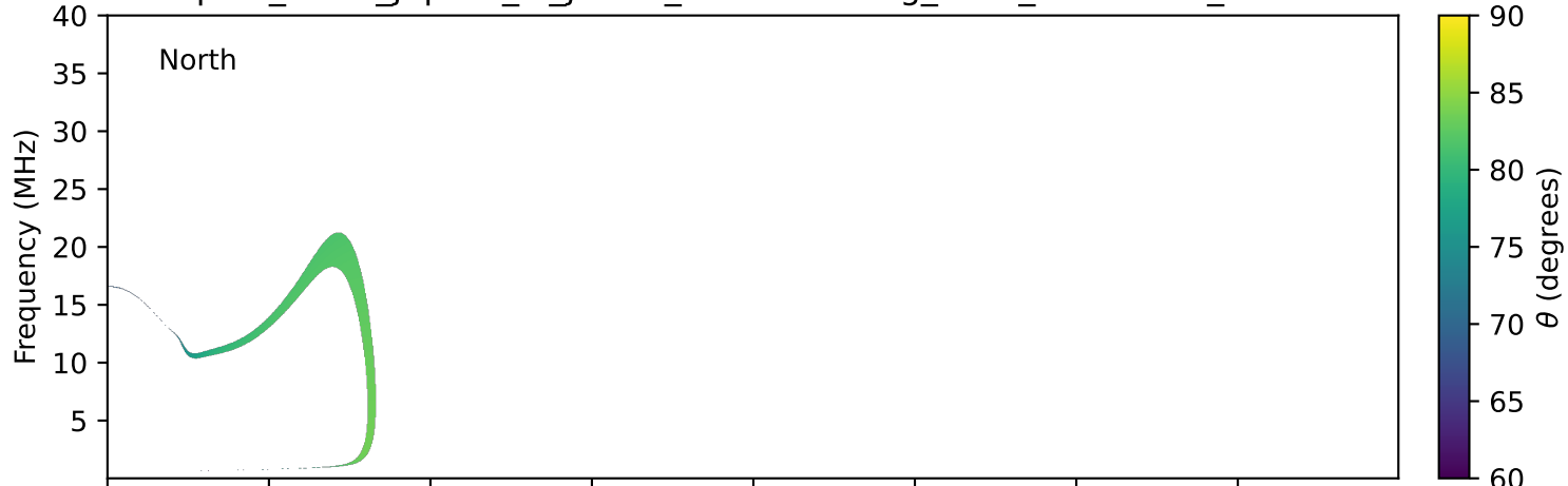
expres_earth_jupiter_io_jrm33_lossc-wid1deg_3kev_20260618_v11.cdf
