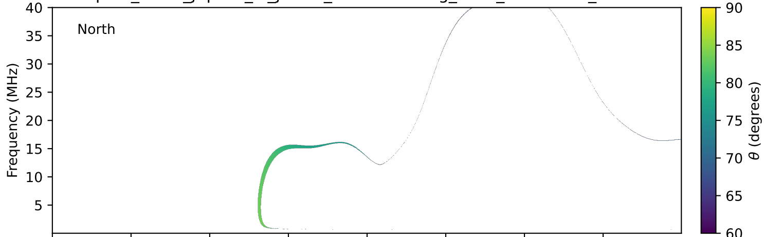
expres_earth_jupiter_io_jrm33_lossc-wid1deg_3kev_20260617_v11.cdf
