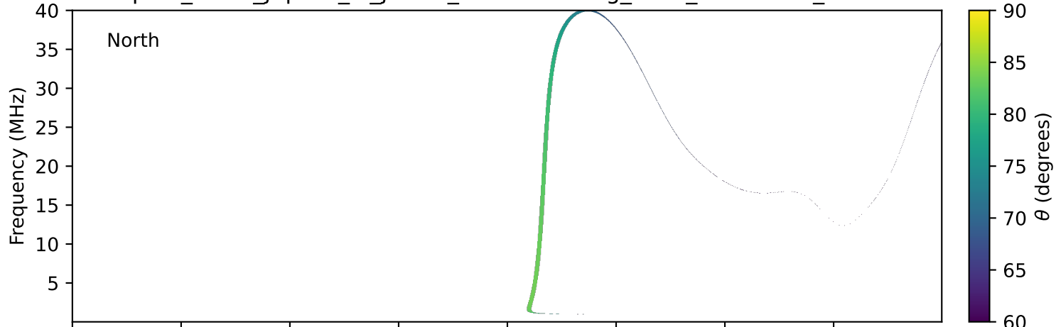
expres_earth_jupiter_io_jrm33_lossc-wid1deg_3kev_20260608_v11.cdf
