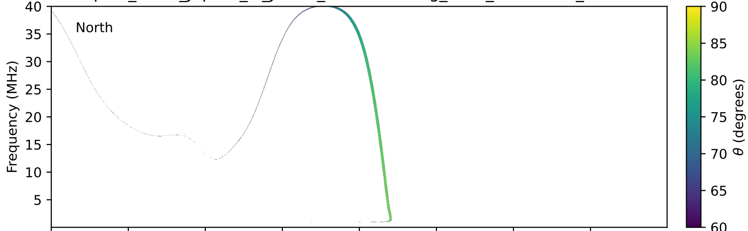
expres_earth_jupiter_io_jrm33_lossc-wid1deg_3kev_20260607_v11.cdf
