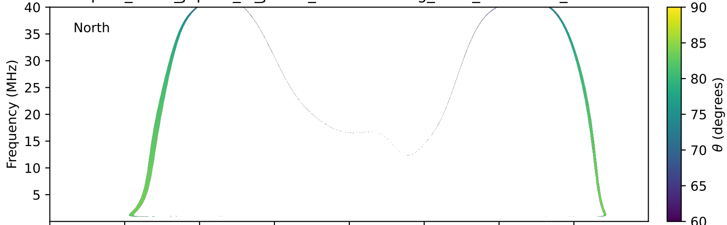
expres_earth_jupiter_io_jrm33_lossc-wid1deg_3kev_20260605_v11.cdf
