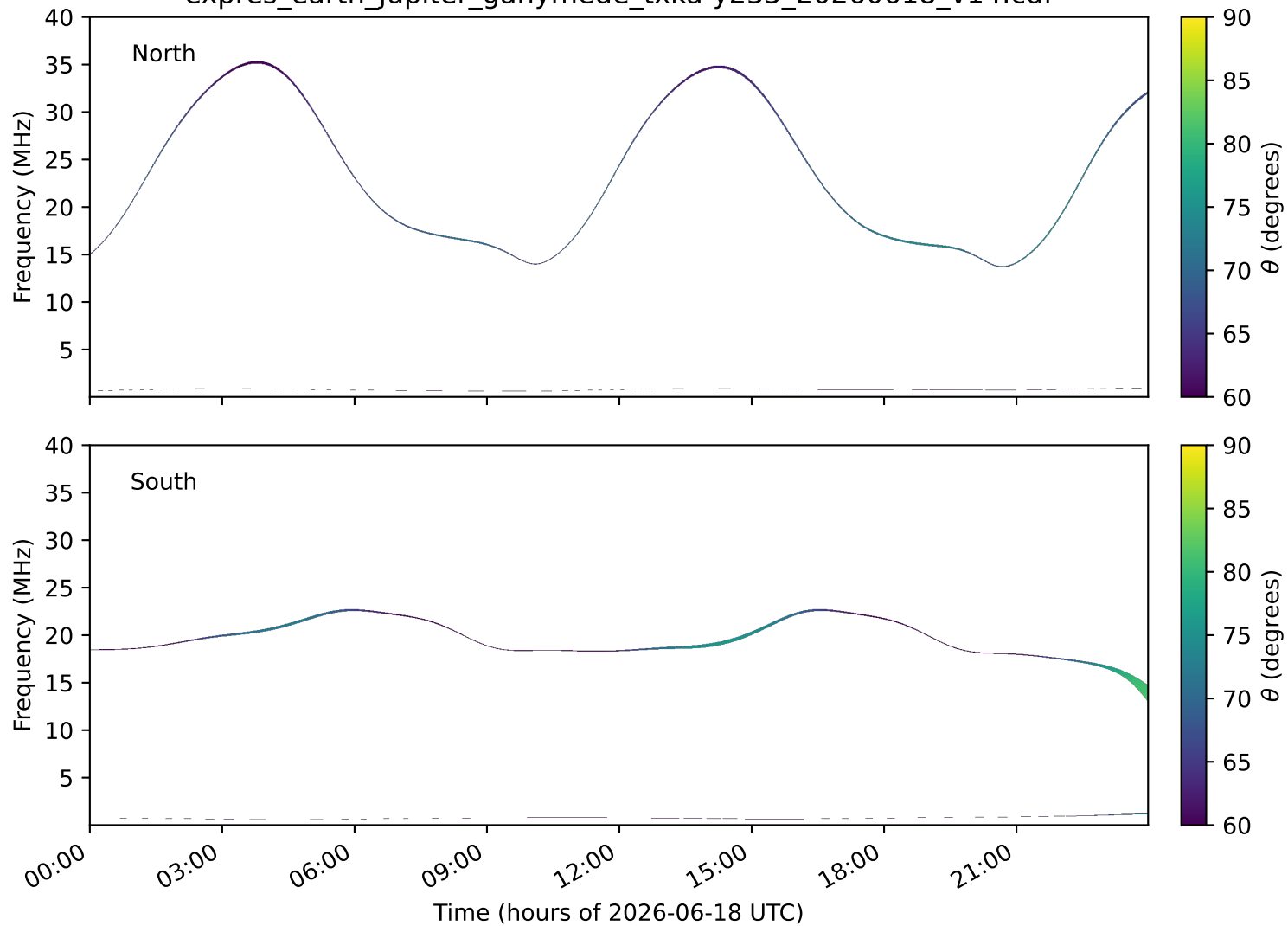
expres_earth_jupiter_ganymede_txka-y235_20260618_v14.cdf
