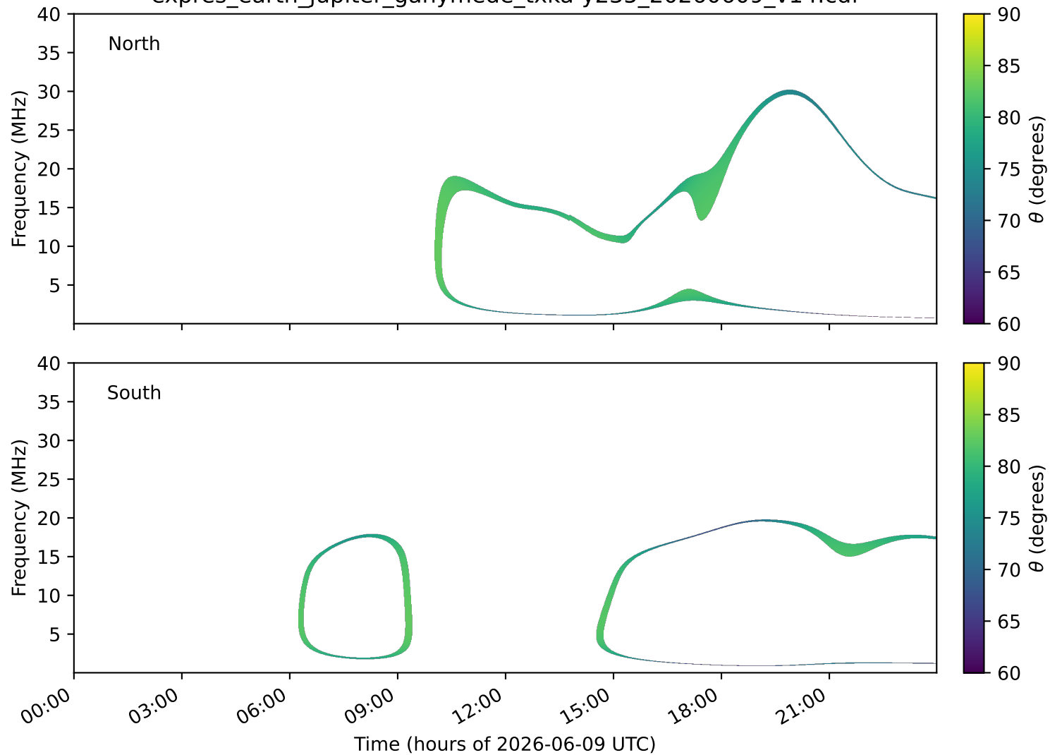
expres_earth_jupiter_ganymede_txka-y235_20260609_v14.cdf
