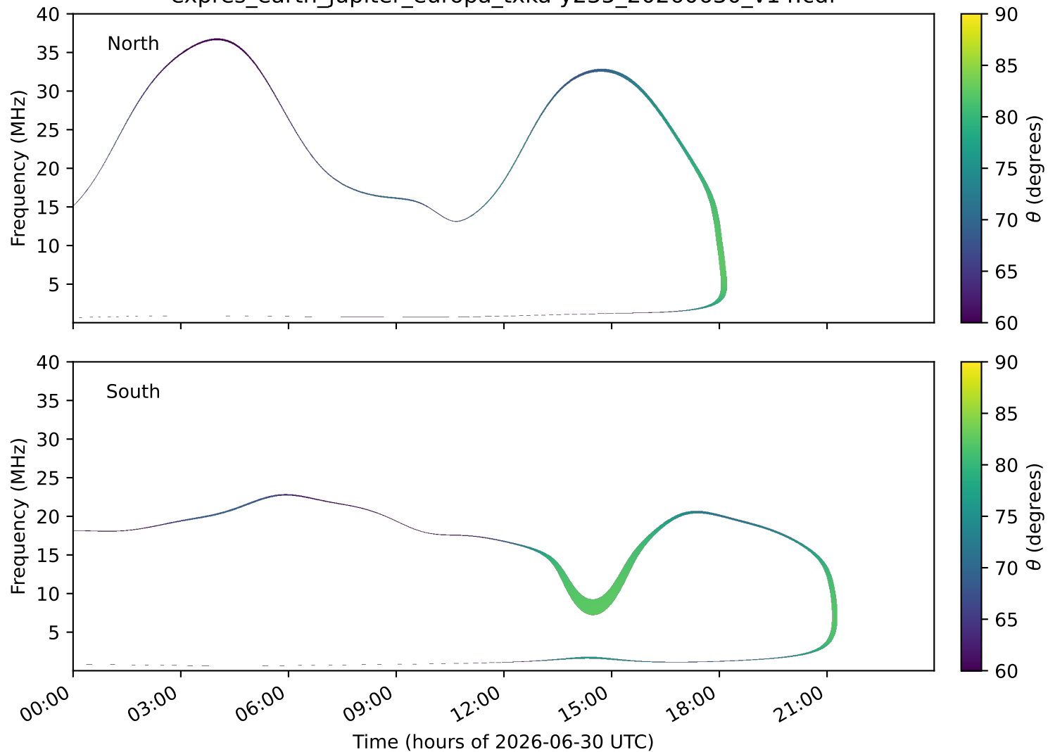
expres_earth_jupiter_europa_txka-y235_20260630_v14.cdf
