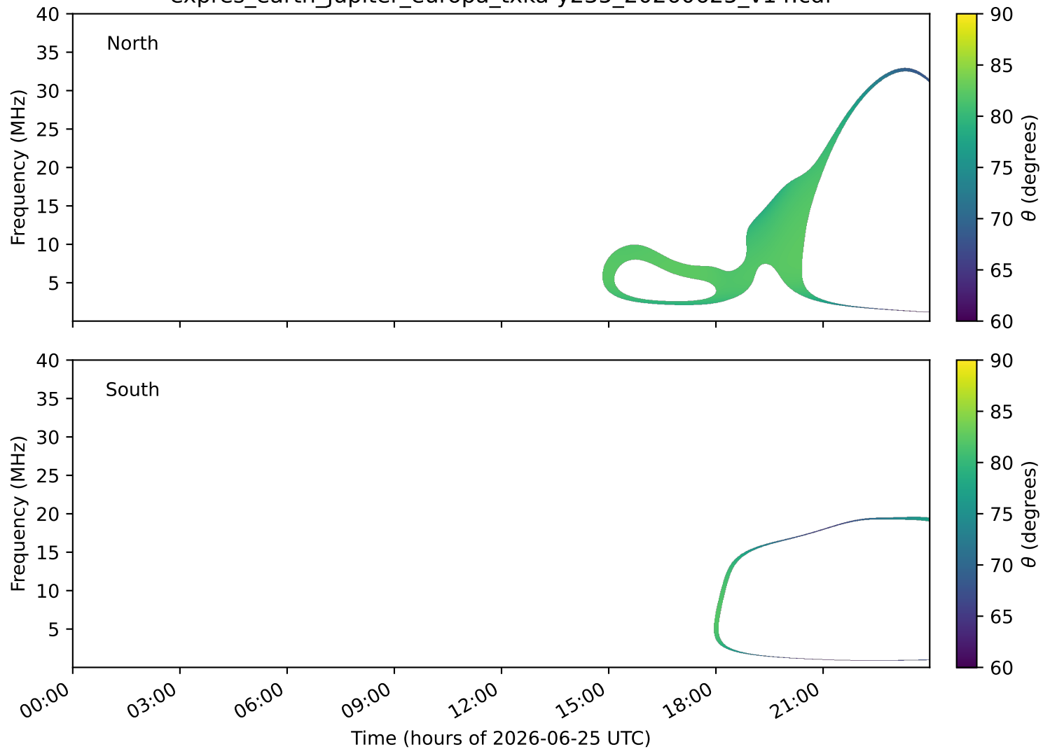
expres_earth_jupiter_europa_txka-y235_20260625_v14.cdf
